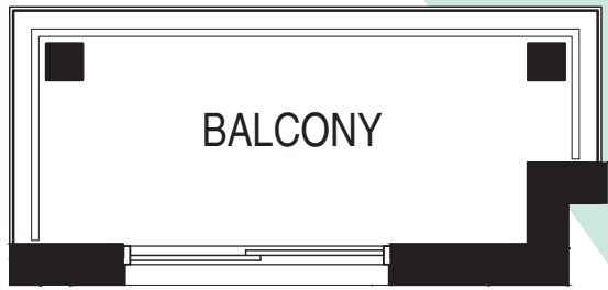
Balcony condition at 4th & 5th Fl. = 66 ft 2
